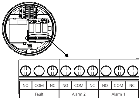
Diagram 15: Relay module with connections shown
